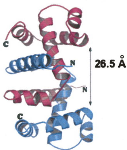
trp aporepressor (no Trp)
